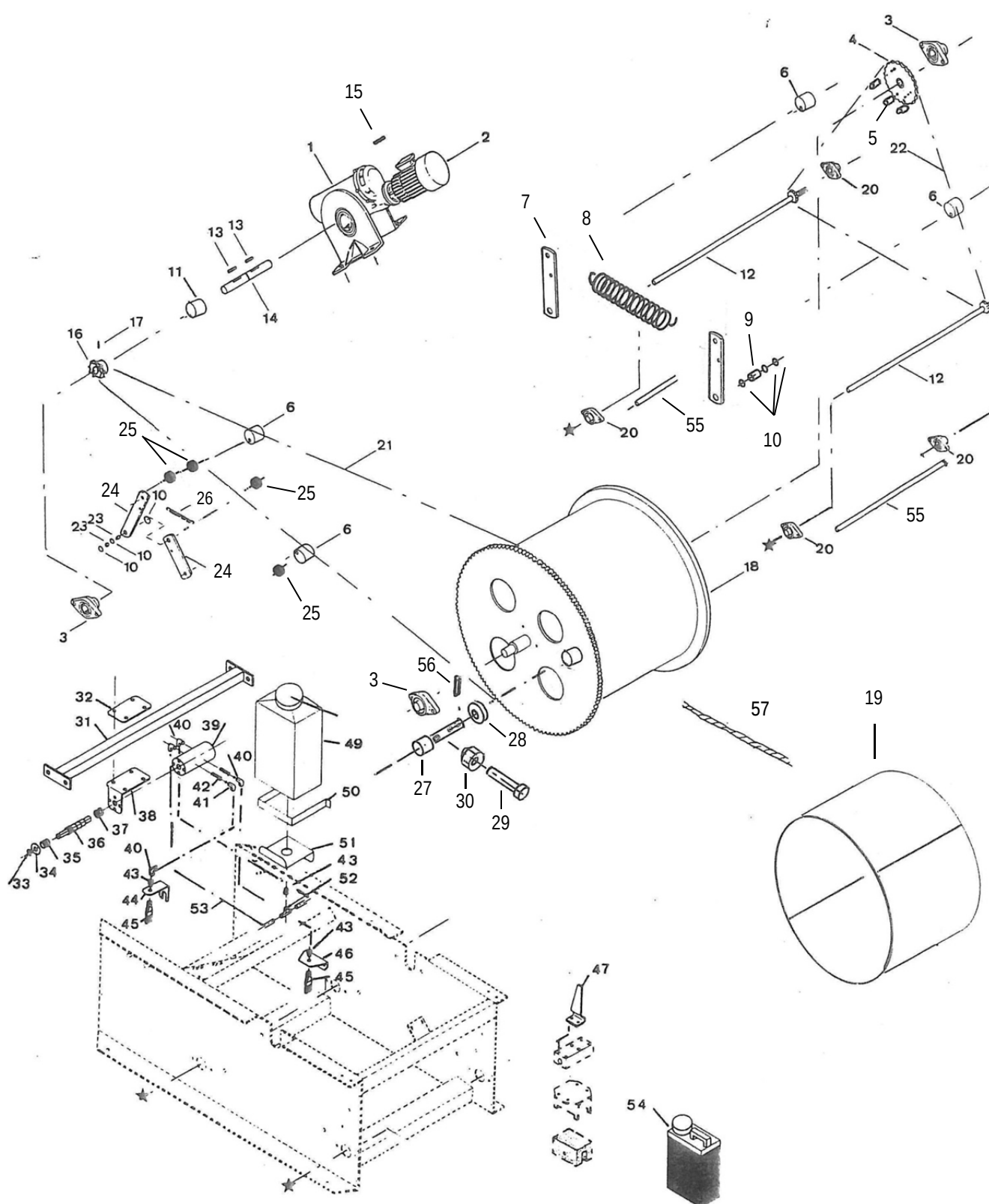
Figure 2. Transmission (2/2)
