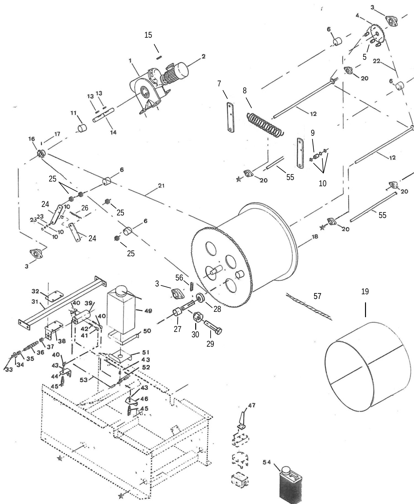
Figure 2. Transmission (1/2)
